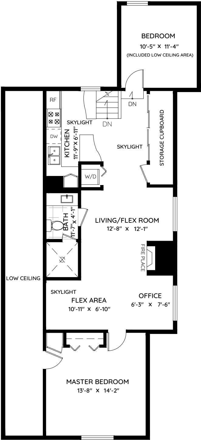
UPPER FLOOR 798 SQ.FT. CH: 8'-2"
