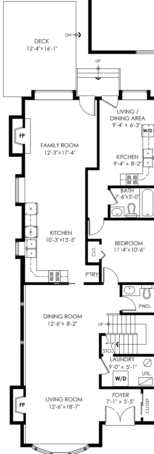
Main Floor Plan Floor Area: 1329 sq.ft.
