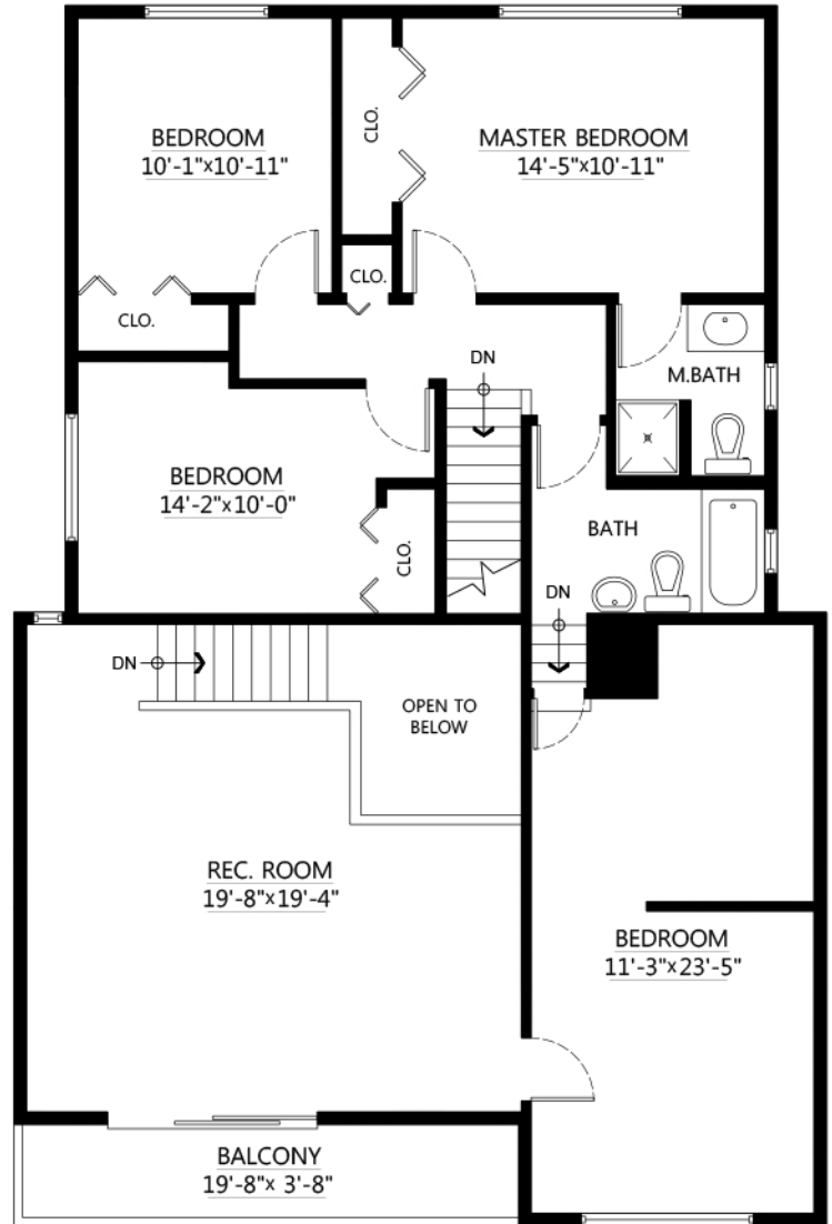
Upper Floor Plan Floor Area: 1335 sq.ft.
