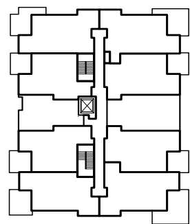
FLOOR LEVEL 1
