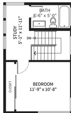
UPPER FLOOR PLAN
