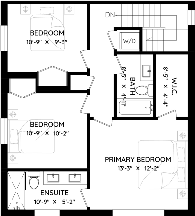
UPPER FLOOR 765 SQ.FT. CH: 12'-0" (VAULTED)
