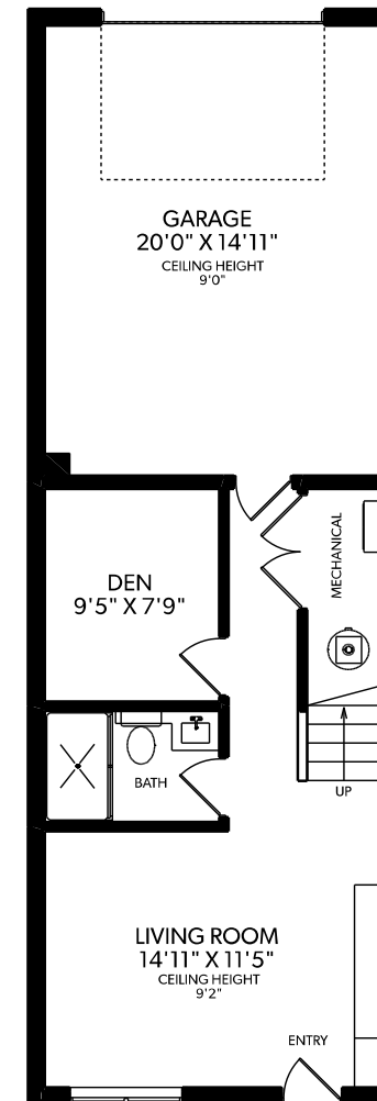
LOWER FLOOR
