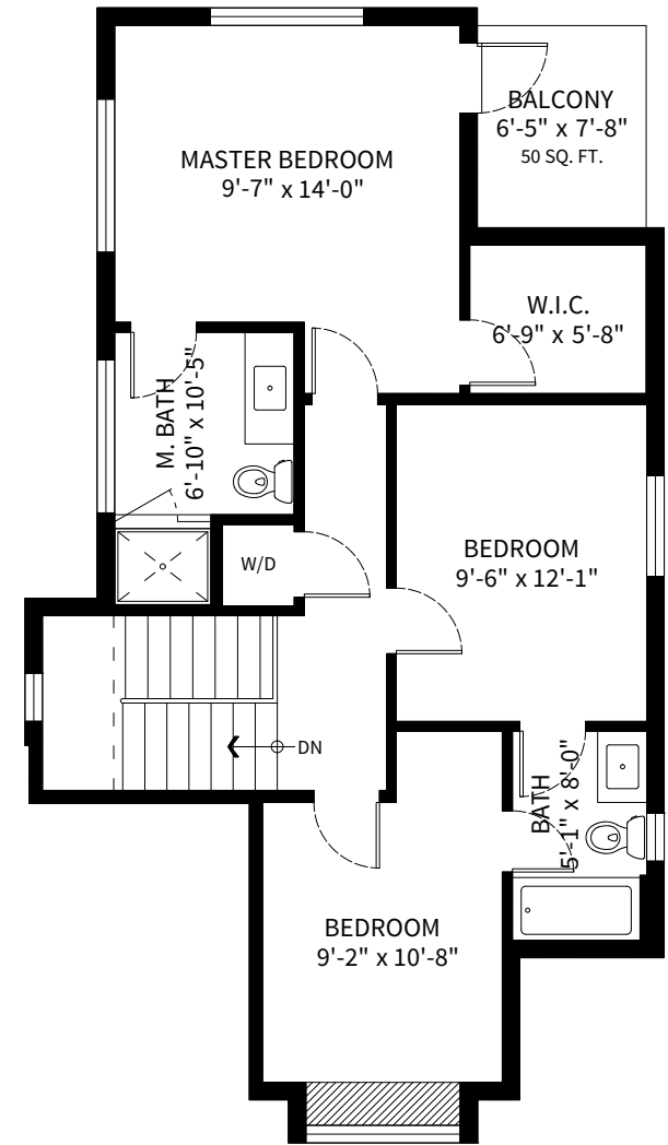
UPPER FLOOR PLAN Ceiling Height: 8'-0"
