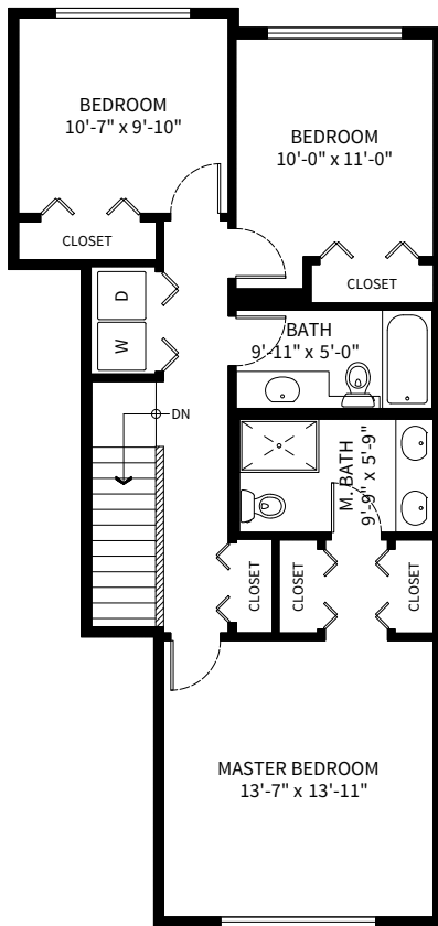
UPPER FLOOR PLAN Ceiling Height: 8'-0"
