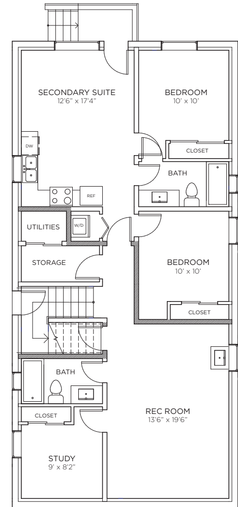
BASEMENT 1,291 SQFT
