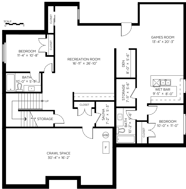
Lower Floor Plan Floor Area: 1,812 sq.ft.
