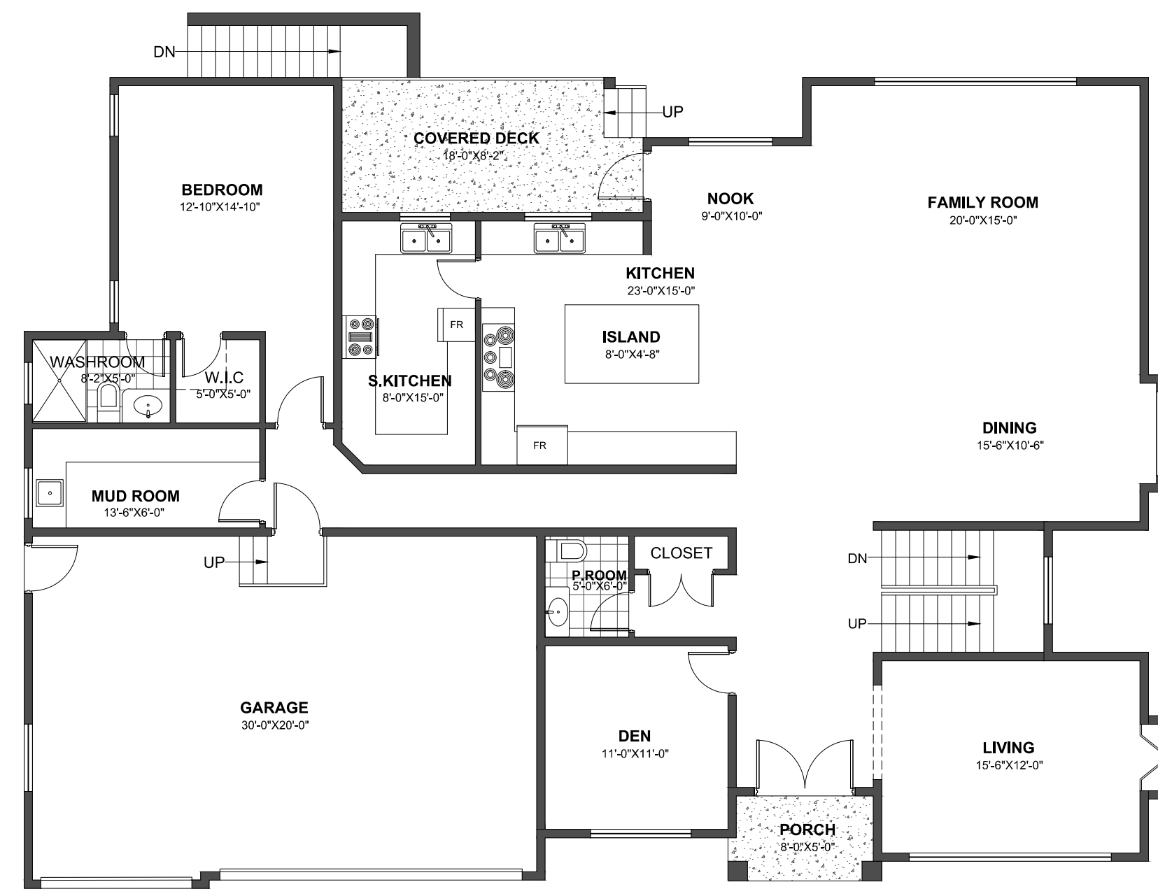
MAIN FLOOR PLAN FLOOR AREA 2823.50 sq.ft
