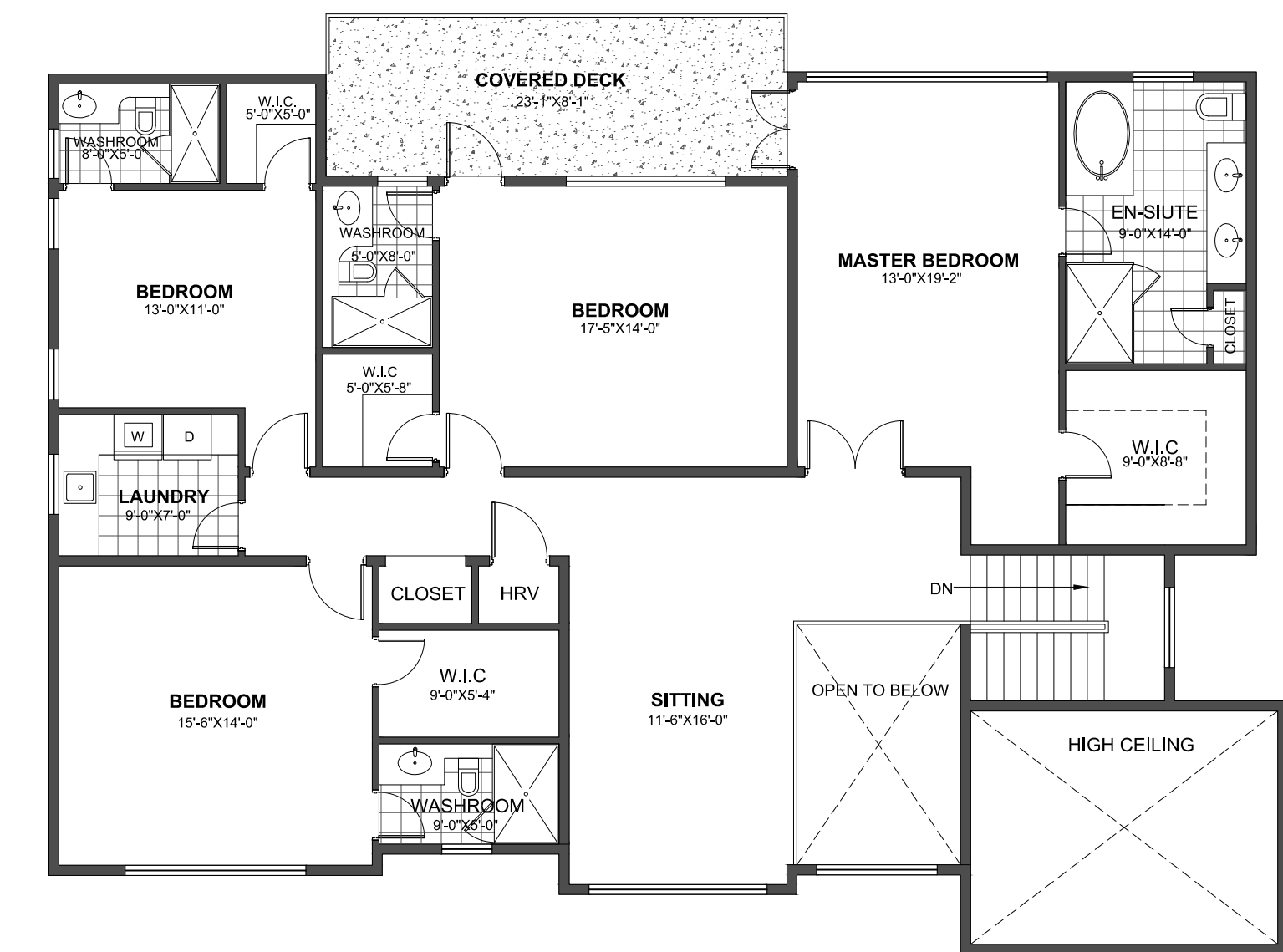
UPPER FLOOR PLAN FLOOR AREA 2145.00sq.ft
