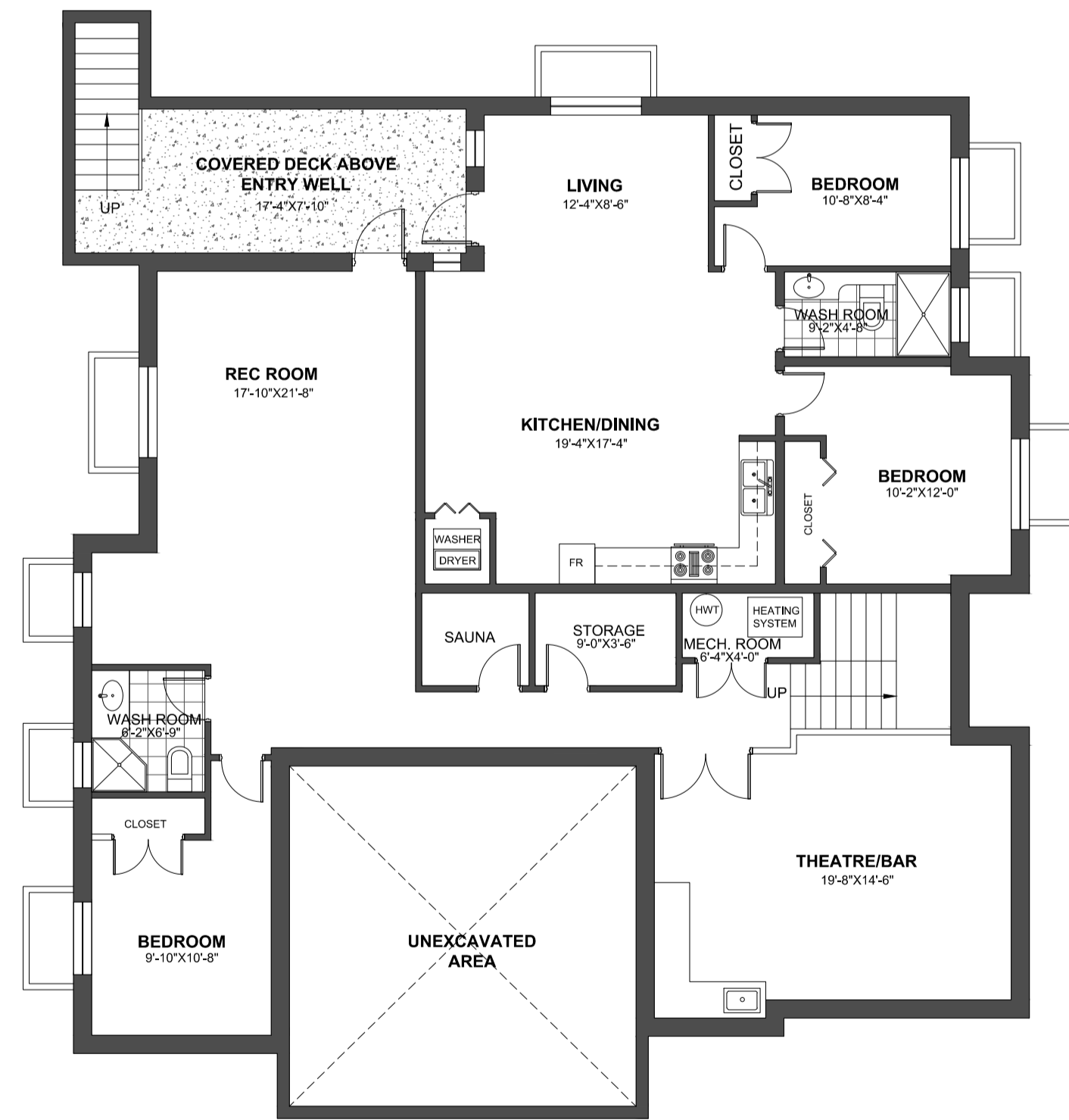
BASEMENT FLOOR PLAN FLOOR AREA 2097.50 sq.ft
