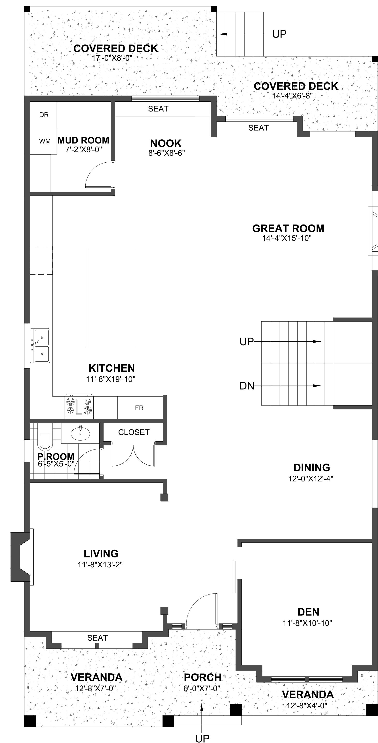
MAIN FLOOR PLAN FLOOR AREA 1540.00 sq.ft
