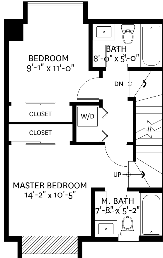
UPPER FLOOR PLAN Ceiling Height: 8'-0"
