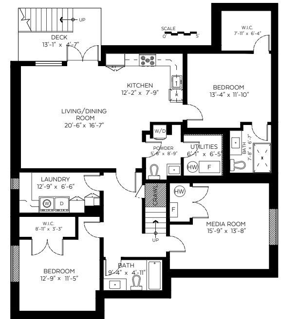
Lower Floor Plan Floor Area: 1,718 sq.ft. Ceiling Height: 8'-5"
