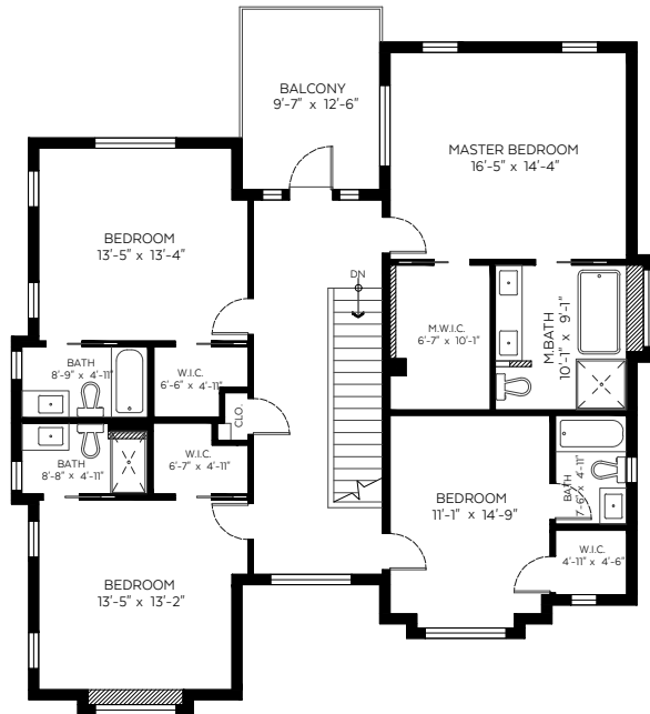
Upper Floor Plan Floor Area: 1,572 sq.ft. Ceiling Height: 8'
