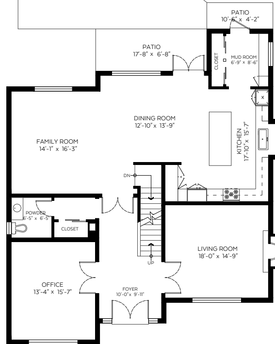
Main Floor Plan Floor Area: 1,718 sq.ft. Ceiling Height: 9'-11"
