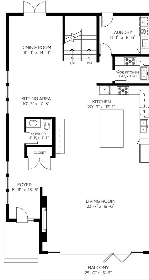
Main Floor Plan Floor Area: 1,668 sq.ft. Ceiling Height: 9'-11"
