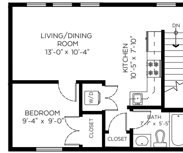
Coach Main Floor Plan Floor Area: 526 sq.ft.
