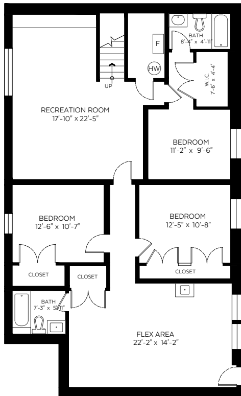
Lower Floor Plan Floor Area: 1,668 sq.ft. Ceiling Height: 9'
