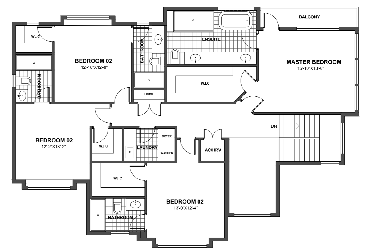
UPPER FLOOR PLAN FLOOR AREA 1562 sq.ft
