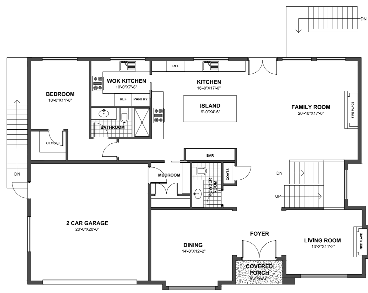
MAIN FLOOR PLAN FLOOR AREA 1724 sq.ft
