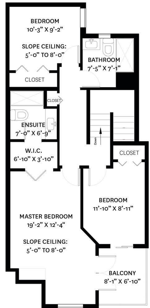
UPPER FLOOR PLAN Ceiling Height: 8'-0"
