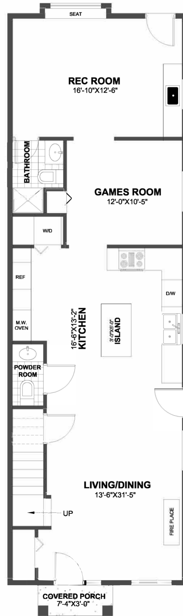
MAIN FLOOR PLAN FLOOR AREA 952.35sq.ft
