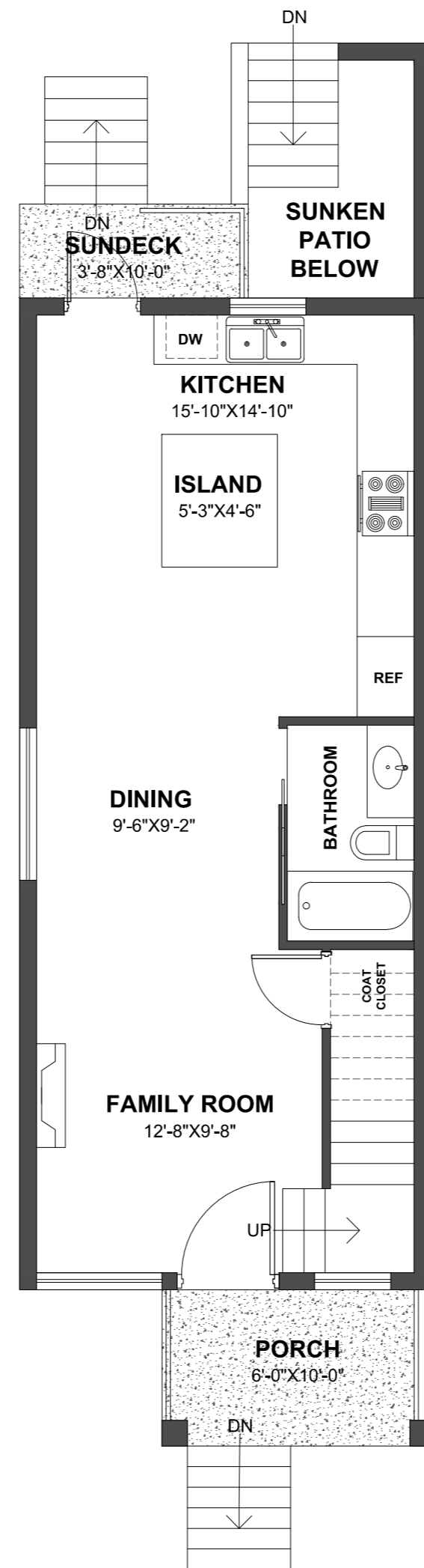
MAIN FLOOR PLAN
