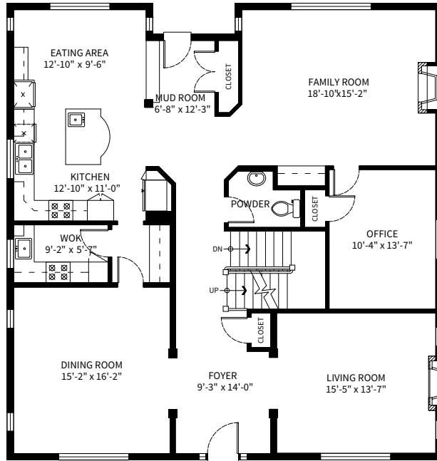
MAIN FLOOR PLAN Ceiling Height: 8'-11"
