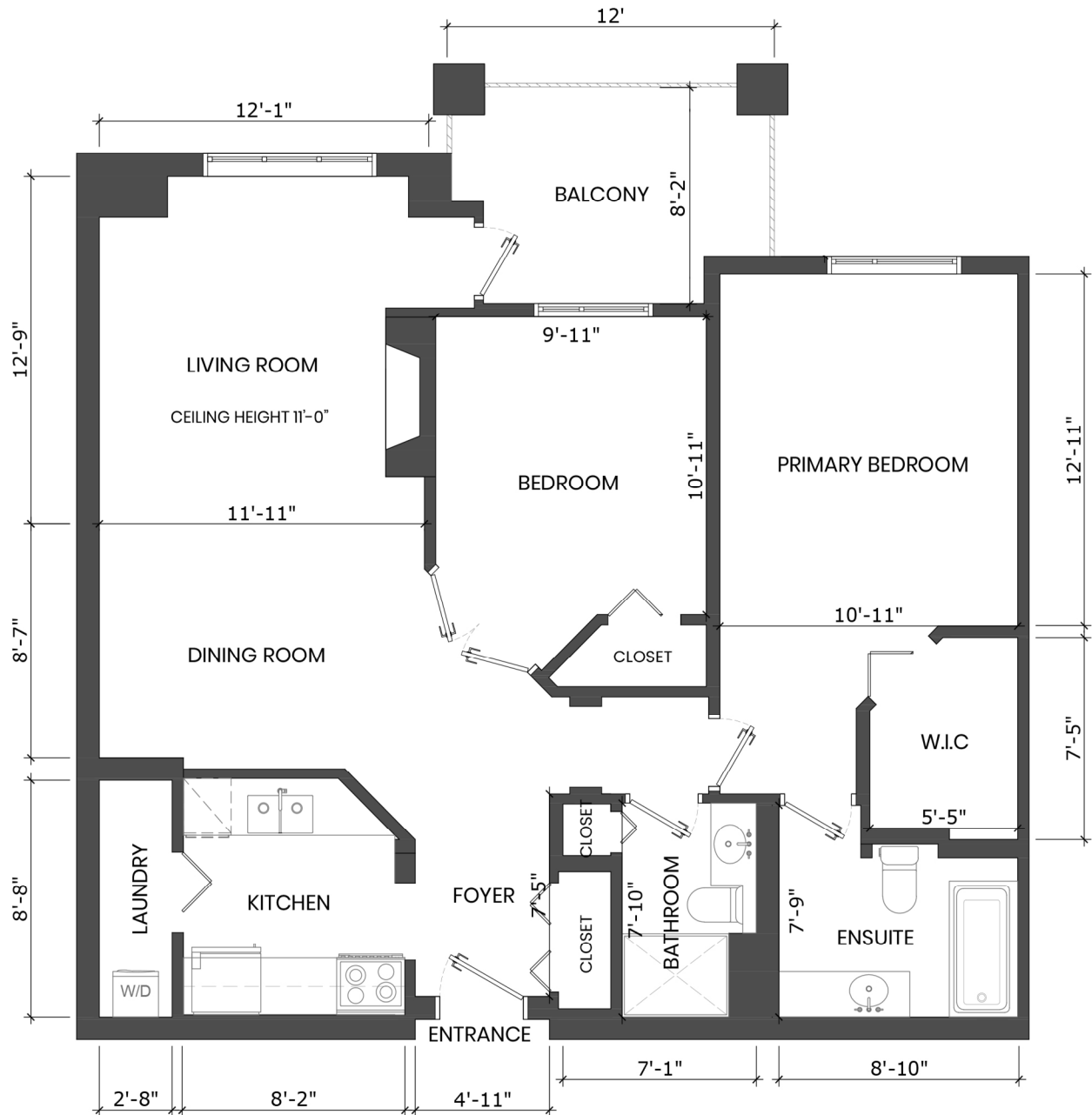
MAIN FLOOR PLAN Ceiling Height: 8'-0"
