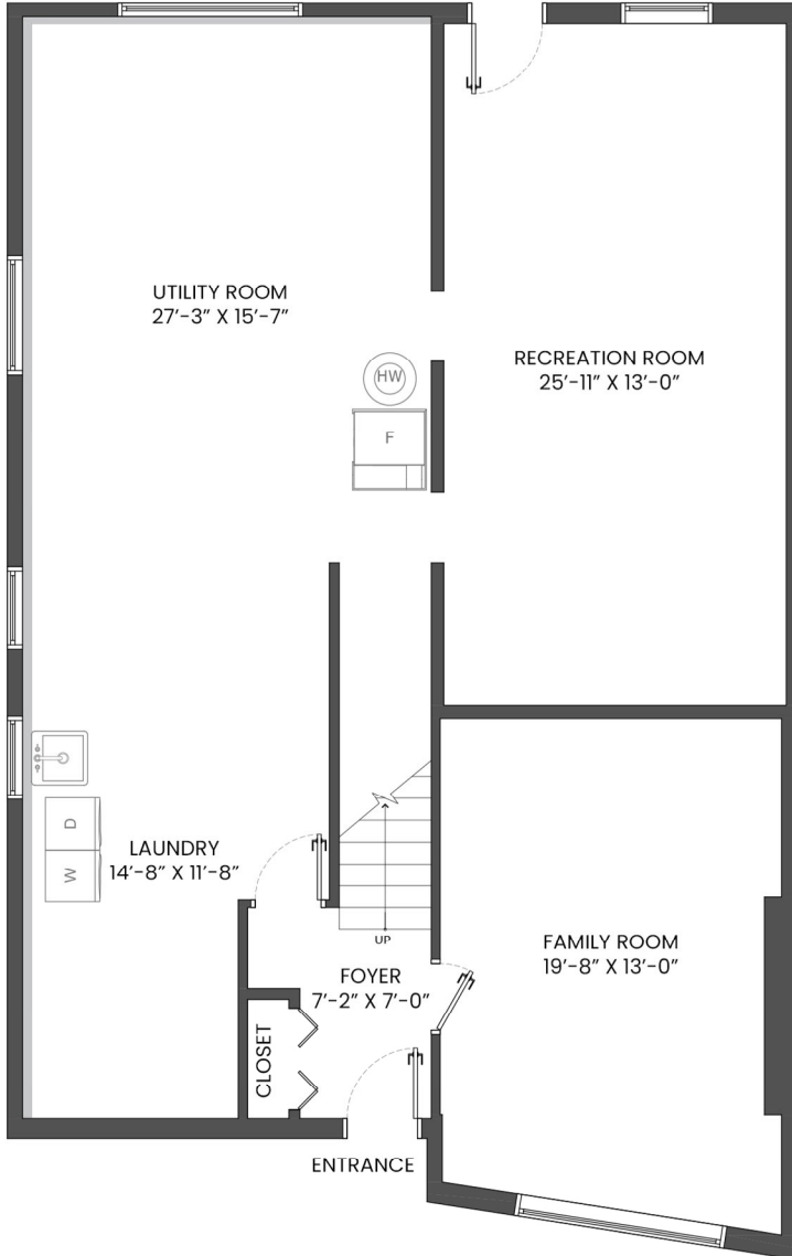
LOWER FLOOR PLAN Ceiling Height: 8'-0"
