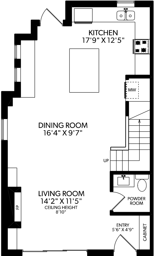
MAIN FLOOR
