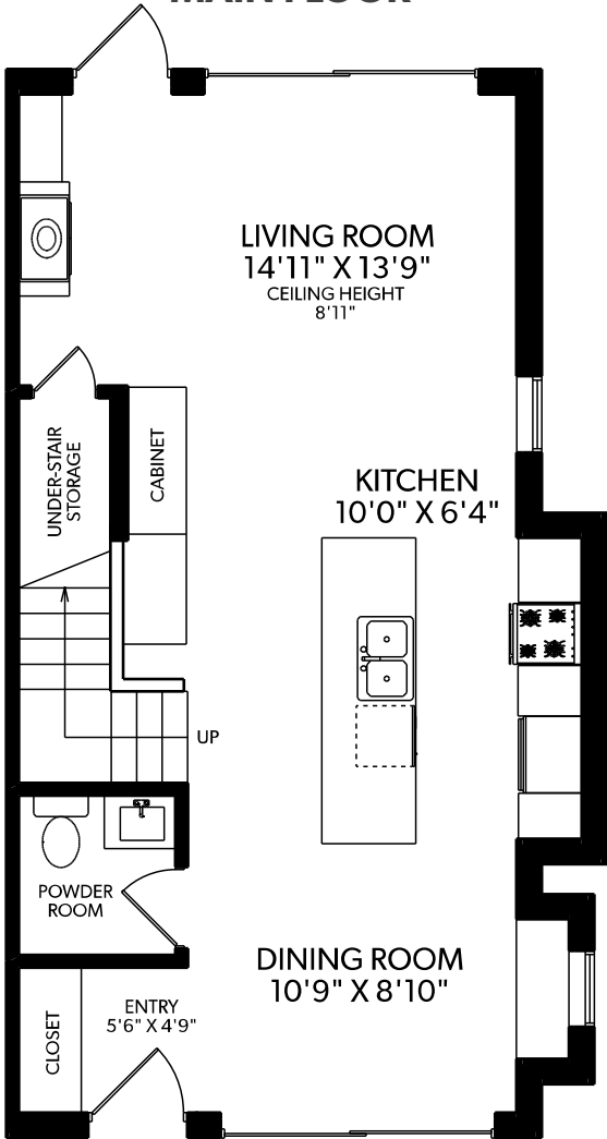
MAIN FLOOR
