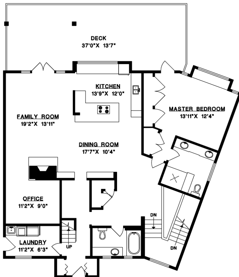
MAIN FLOOR
