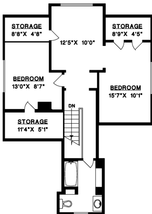
UPPER FLOOR
