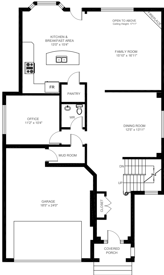
MAIN FLOOR ( 1287 sq.ft.) Ceiling Height: 9'
