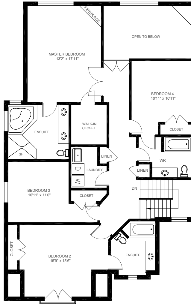
SECOND FLOOR ( 1728 sq.ft.) Ceiling Height: 8'
