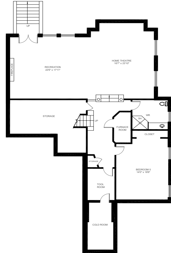
LOWER FLOOR ( 2088 sq.ft.)
