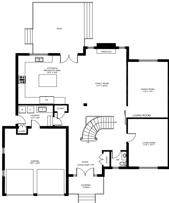
MAIN FLOOR ( 1520 sq.ft.) Ceiling Height: 9'
