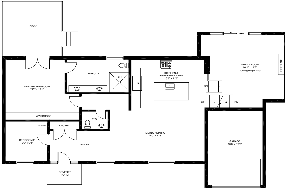
MAIN FLOOR (1,550 sq.ft.) Ceiling Height: 8'0"
