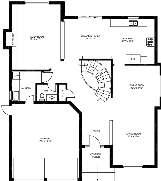
MAIN FLOOR (1,340 sq.ft.) Ceiling Height: 9'
