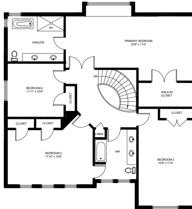
SECOND FLOOR (1,497 sq.ft.) Ceiling Height: 8'
