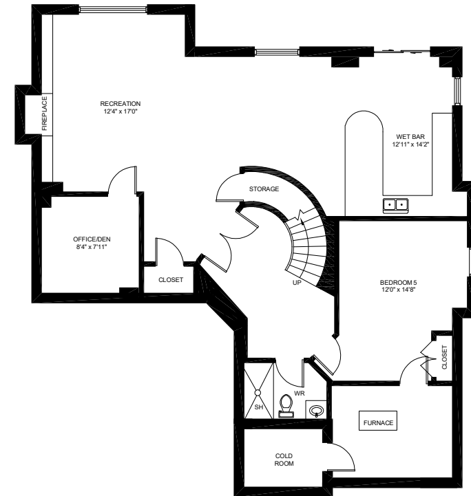
LOWER FLOOR (1,400 sq.ft.) Ceiling Height: 8'2"
