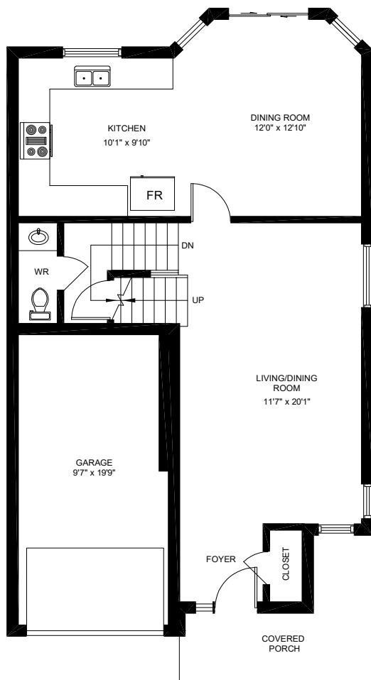
MAIN FLOOR (702 sq.ft.) Ceiling Height: 8'
