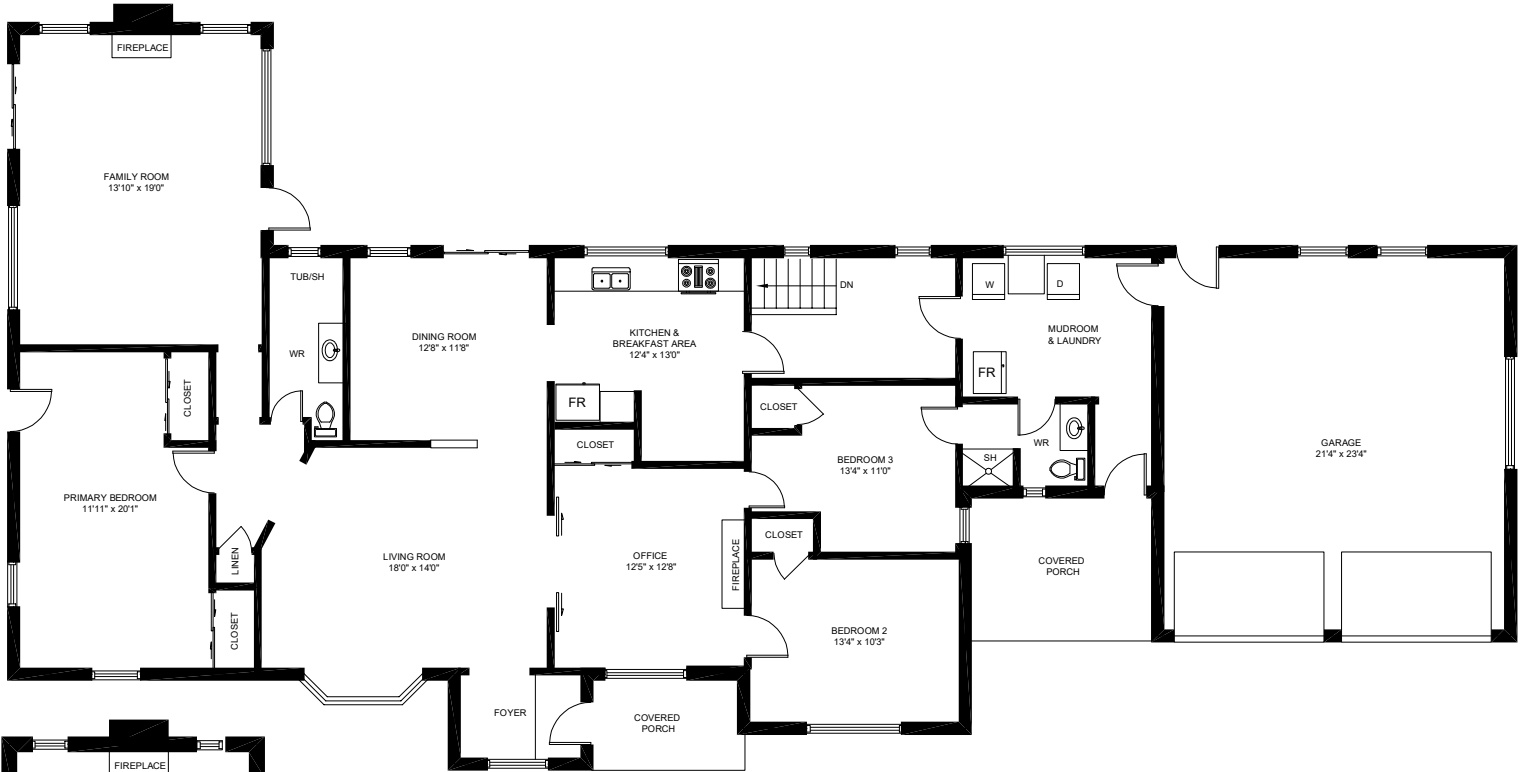
MAIN FLOOR (2,100 sq.ft.) Ceiling Height: 8'
