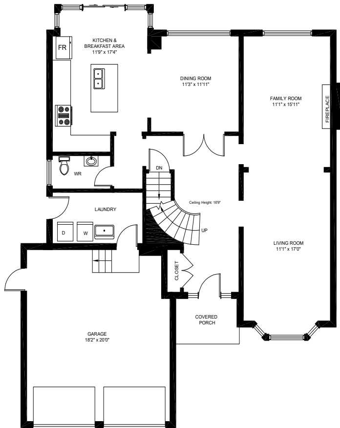
MAIN FLOOR (1,165 sq.ft.) Ceiling Height: 8'
