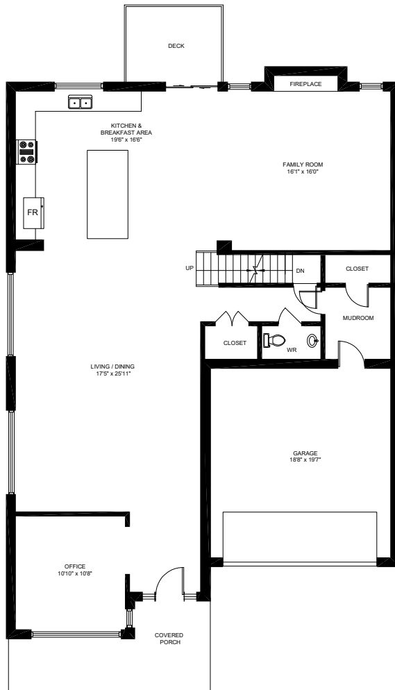
MAIN FLOOR (1,604 sq.ft.) Ceiling Height: 10'
