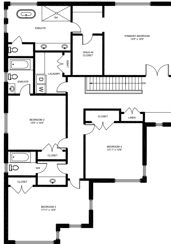
SECOND FLOOR (1,783 sq.ft.) Ceiling Height: 9'
