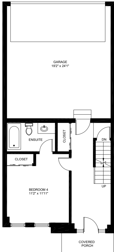
FIRST FLOOR (402 sq.ft.) Ceiling Height: 9'
