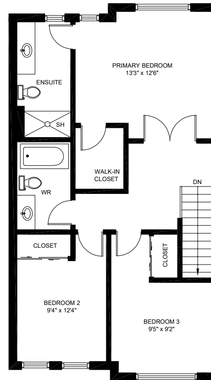
THIRD FLOOR (732 sq.ft.) Ceiling Height: 8'
