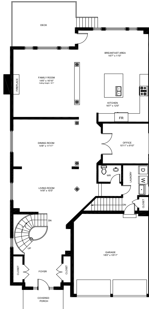
MAIN FLOOR (1,808 sq.ft.) Ceiling Height: 9'
