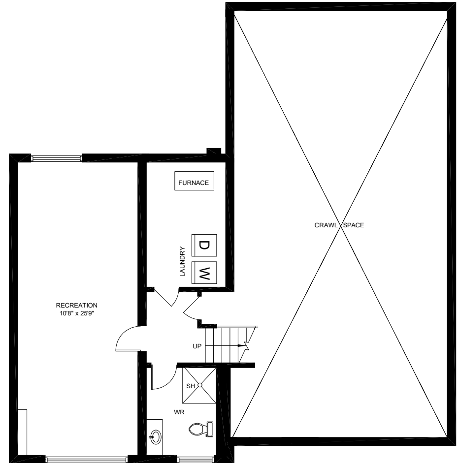
LOWER FLOOR (556 sq.ft.) Ceiling Height: 7'1"
