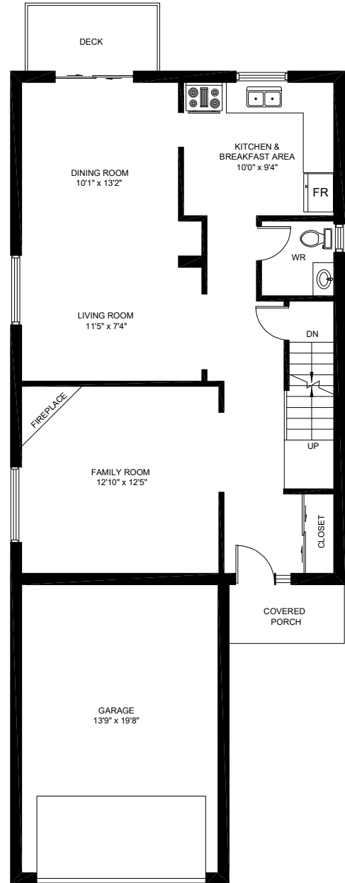
MAIN FLOOR (773 sq.ft.) Ceiling Height: 8'
