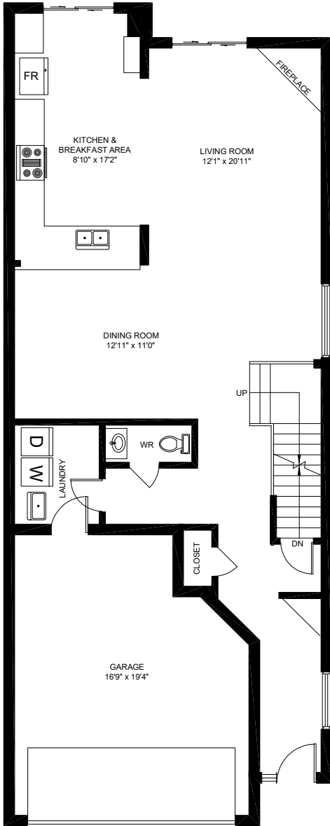
MAIN FLOOR (950 sq.ft.) Ceiling Height: 9'
