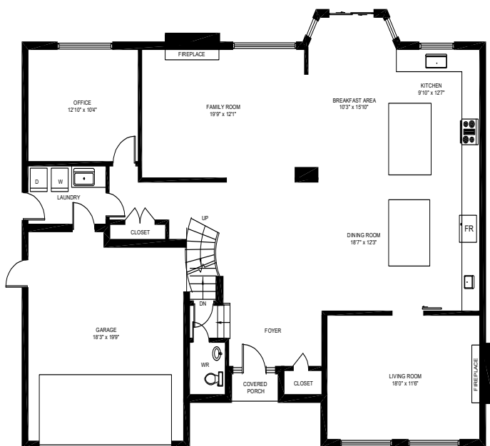
MAIN FLOOR (1,688 sq.ft.) Ceiling Height: 8'4"
