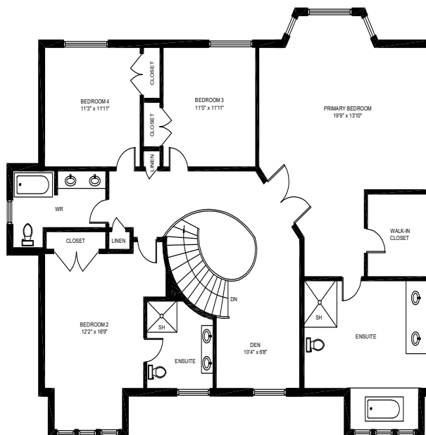
SECOND FLOOR (1,717 sq.ft.) Ceiling Height: 8'0"
