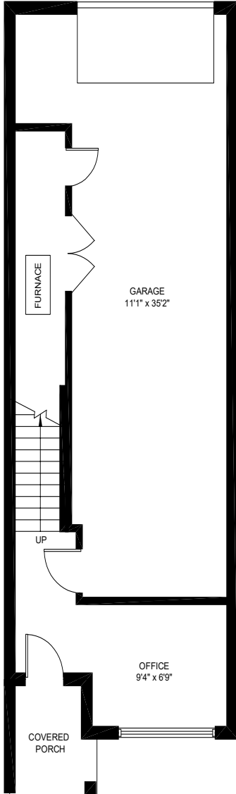
MAIN FLOOR (159 sq.ft.)
