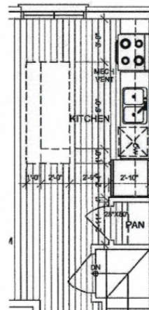
FLOOR PLAN - ALT KITCHEN
