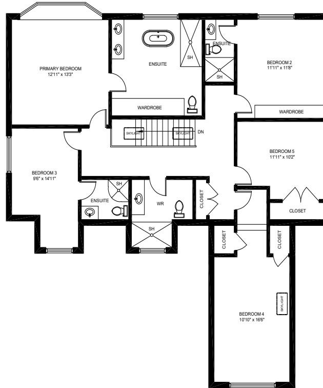
SECOND FLOOR (1,375 sq.ft.) Ceiling Height: 8'
