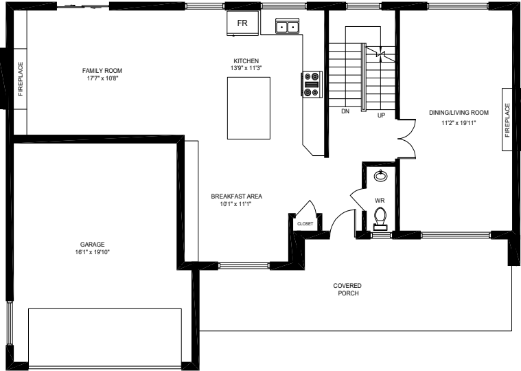
MAIN FLOOR Ceiling Height: 8'
