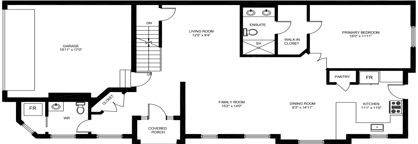
MAIN FLOOR (1,235 sq.ft.) Ceiling Height: 9'
