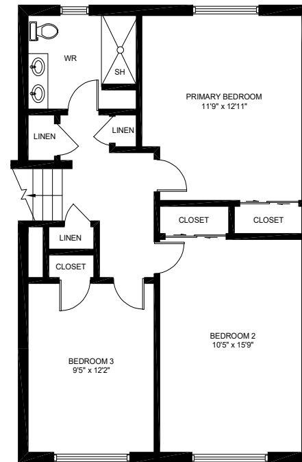
SECOND FLOOR (720 sq.ft.) Ceiling Height: 8'
