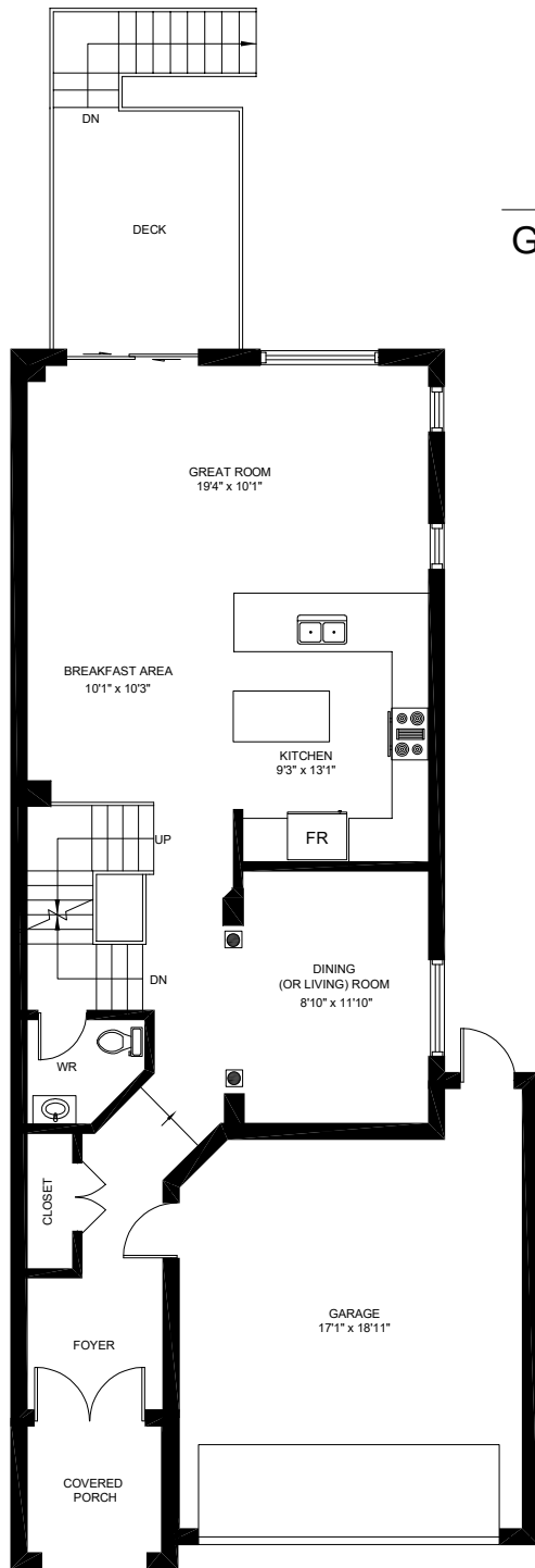
MAIN FLOOR (882 sq.ft.) Ceiling Height: 9'
