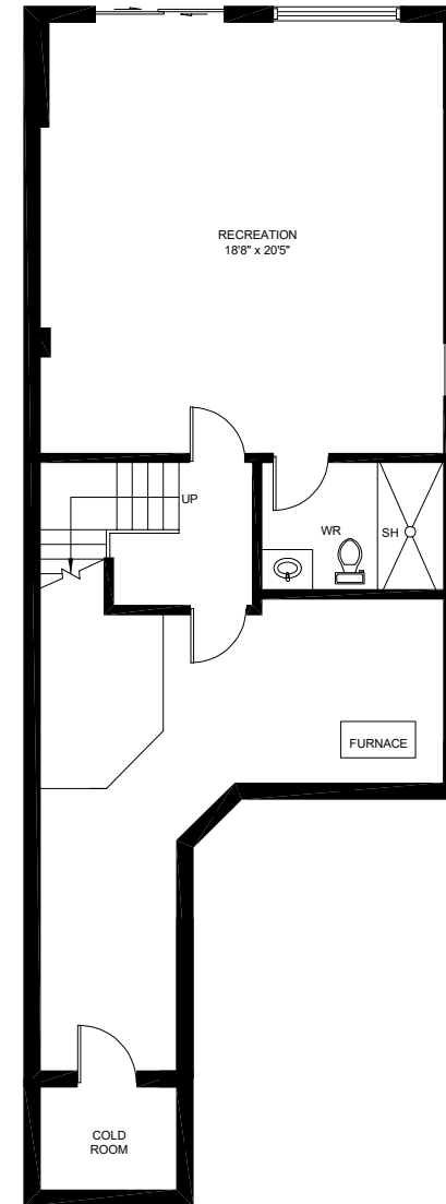
LOWER FLOOR (932 sq.ft.) Ceiling Height: 8'1"
