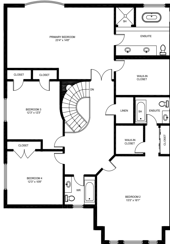
SECOND FLOOR (1,708 sq.ft.) Ceiling Height: 8'
